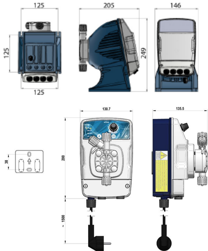
Fig. 1 - Dimensions in mm. Plate for wall mounting.
