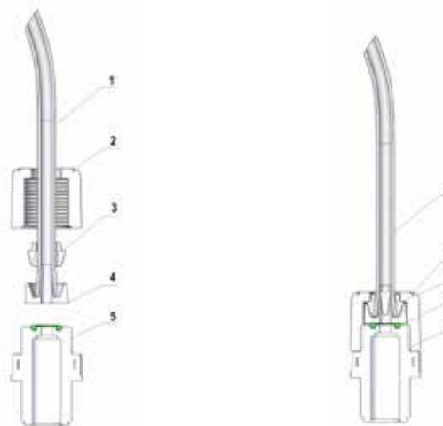
Fig.4 - Raccordement hydraulique
