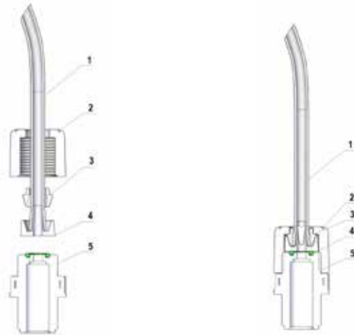
Fig.4 – Hydraulic Connection
