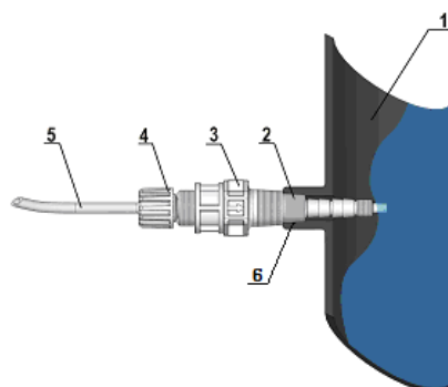
Fig. 7 - Connection assembly
