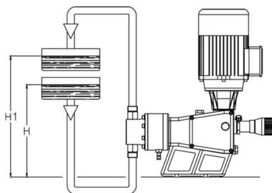
Fig. 6.1 installation idéale
