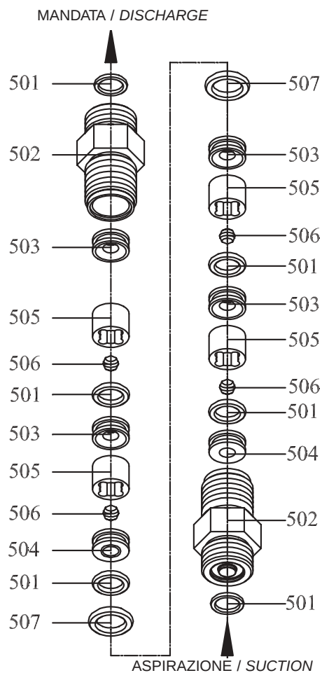
DOPPIA VALVOLA DOUBLE VALVE ASSEMBLY VALVULA DOBLE
