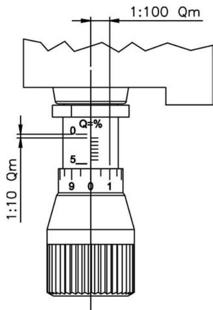
Fig. 16 – Micrometer adjustment
