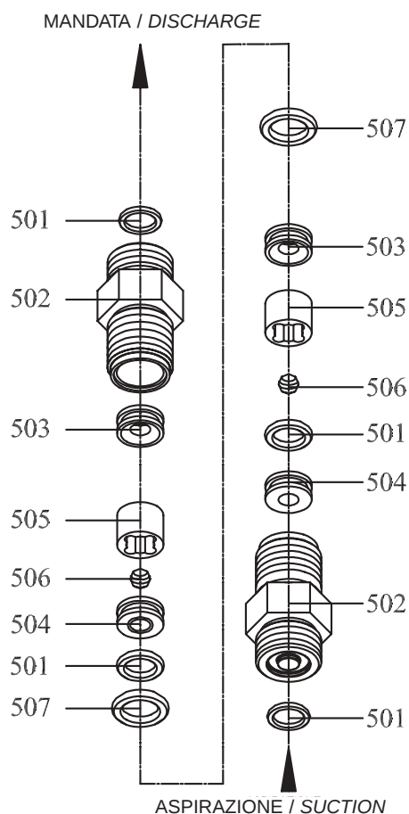
SINGOLA VALVOLA SINGLE VALVE ASSEMBLY VALVULA SIMPLE
