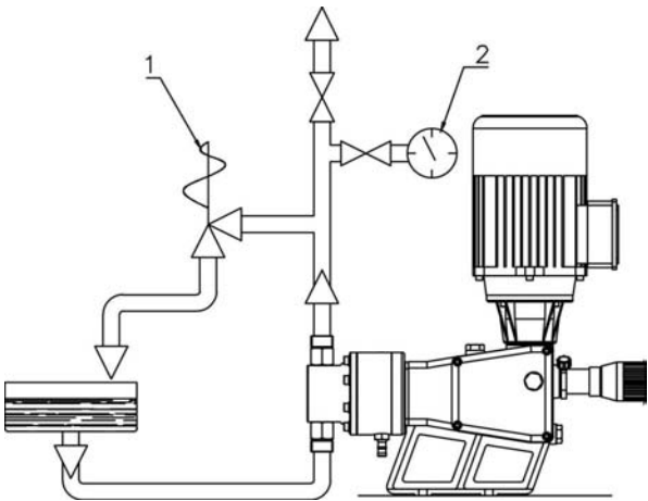
Fig. 7 – Safety valves
